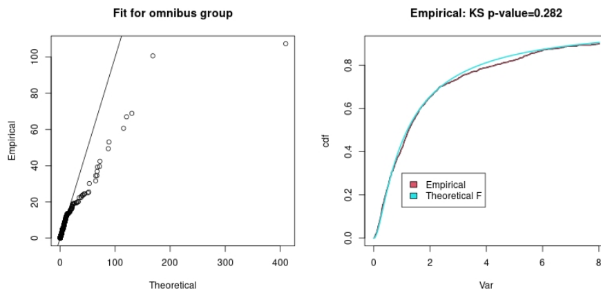
Figure 11: An output from the anota2seqPerformQC function (used with parameter useRVM = TRUE ) comparing obtained variances to the theoretical F-distribution. RVM assumes that the empirical and the theoretical distributions are similar. A Kolmogorov-Smirnov test is used to assess a difference between the distributions and the p-value is indicated. Data sets with small deviations where lines largely overlap albeit with a, for a Kolmogorov-Smirnov test on thousands of data points, modest p-value (e.g. larger than approximately 0.001) are considered fit for further analysis.
