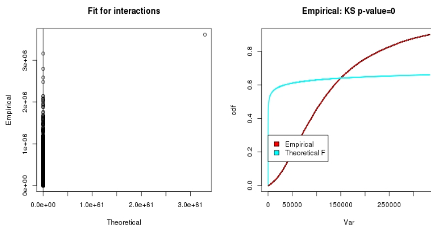
Figure 10: An output from the anota2seqPerformQC function (used with parameter useRVM = TRUE ) comparing obtained variances to the theoretical F-distribution for a poor-quality data set. RVM assumes that the empirical and the theoretical distributions are similar. Notice the strong difference between the expected theoretical and obtained distributions. A Kolmogorov-Smirnov test is used to assess a difference between the distributions and the p-value is indicated. Data sets with small deviations where lines largely overlap albeit with a, for a Kolmogorov-Smirnov test on approximately 10 000 data points, modest p-value (e.g. larger than approximately 0.001) are considered fit for further analysis.
